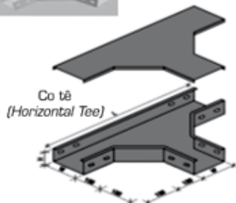
Nắp Co tê (Horizontal Tee Cover)
