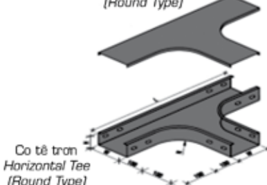
Nắp Co tê trơn Horizontal Tee Cover (Round Type)
